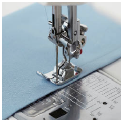
200-125-020 Straight stitch foot
